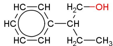
2-phenylbutan-1-ol
