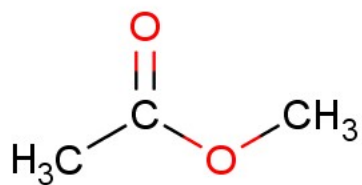
Methylethanoat
