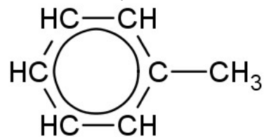
Methylbenzen
