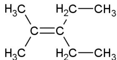
3-ethyl-2-methylpent-2-en
