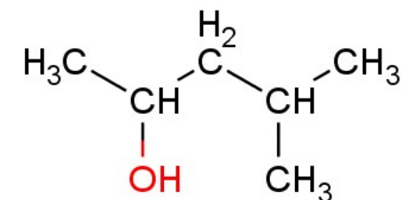
4-methylpentan-2-ol
