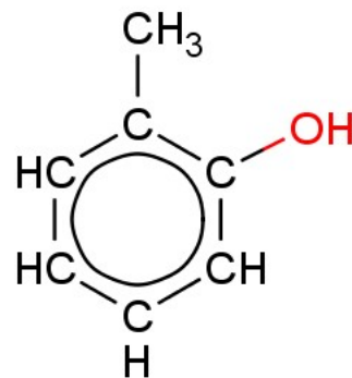
2-methylphenol
