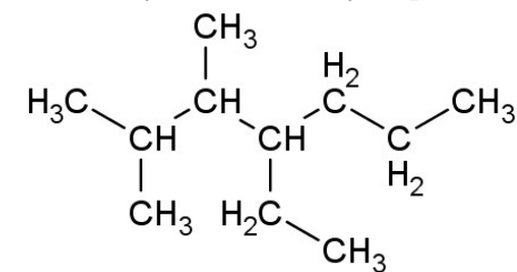
4-ethyl-2,3-dimethylheptan
